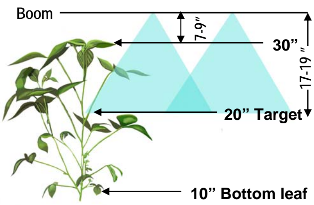
Figure 1. Height adjustment for a spray boom equipped with 80 degree flat fan nozzles spaced at 20" and used in 30" tall soybeans
